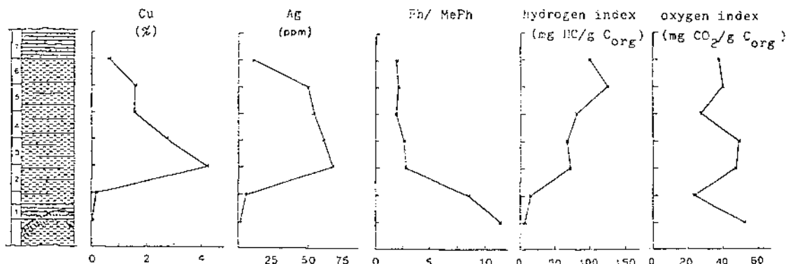
Figure 2: Variation of the copper content (%), the silver content (ppm), the hydrogen index (HI measured as mg HC/g C org ) and the ratio of phenanthrene/sum of methylphenanthrenes (Ph/ \Sigma MePh) in the seven samples of profile no. 1 from Kupferschiefer and adjacent rocks (Konrad mine).
