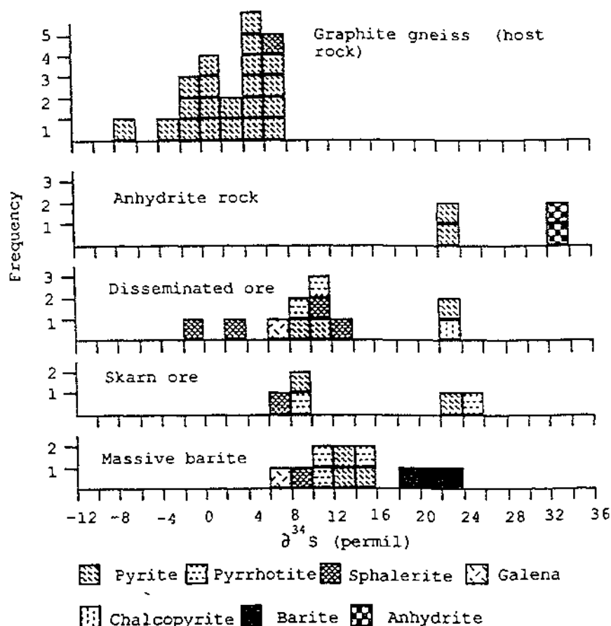
Fig.2. Isotopic composition of sulphides, barite and anhydrite from the Rožná host-rock graphitic gneiss, anhydrite lens, massive barite ore, disseminated and skarn ore
