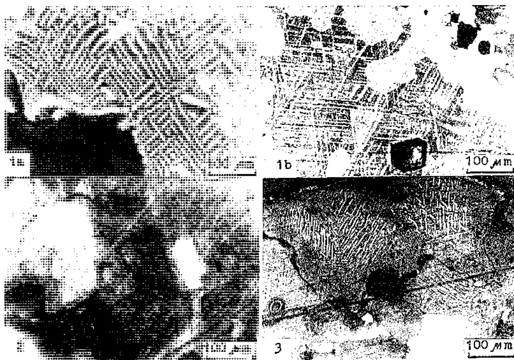
Fig 1. Lamellar systems of AuCu- (white) and Au,Ag' (grey) - phases.
