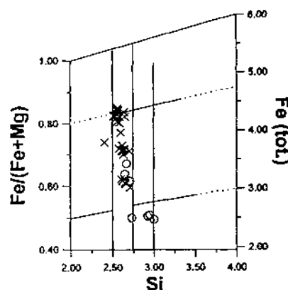
Fig. 3. EMP trioctahedral Chlorite compositions in Hey's diagram. Crosses: Masa Valverde footwall chlorites. Circles: Riotinto stockwork chlorites.
