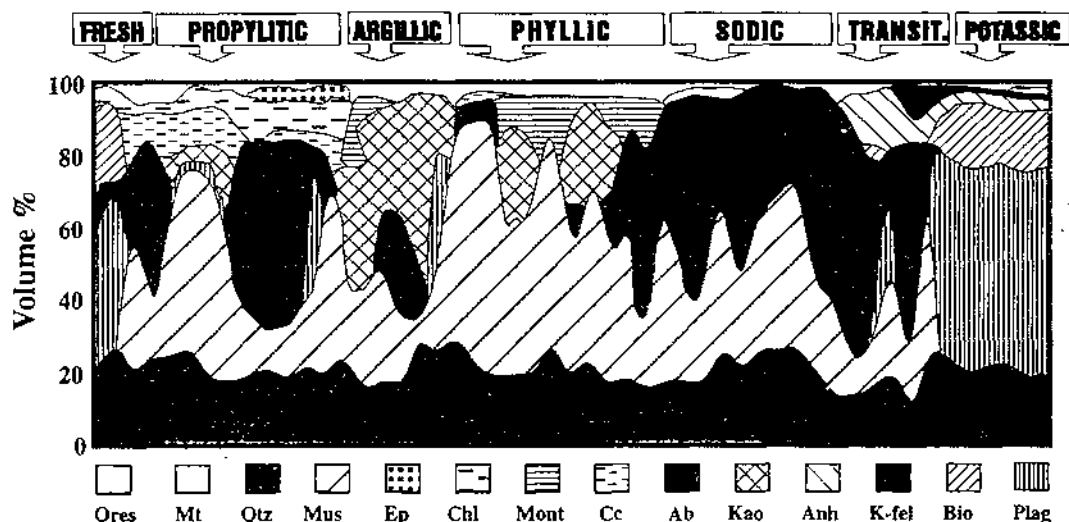
FIG. 1. An idealized section across the deposit showing the distribution of the major primary and secondary minerals. Mineral abundances were calculated using a linear least square regression method relating whole-rock chemical analyses to the products of the amount and composition of the constituent mineral phases (Böhlke, 1989).
