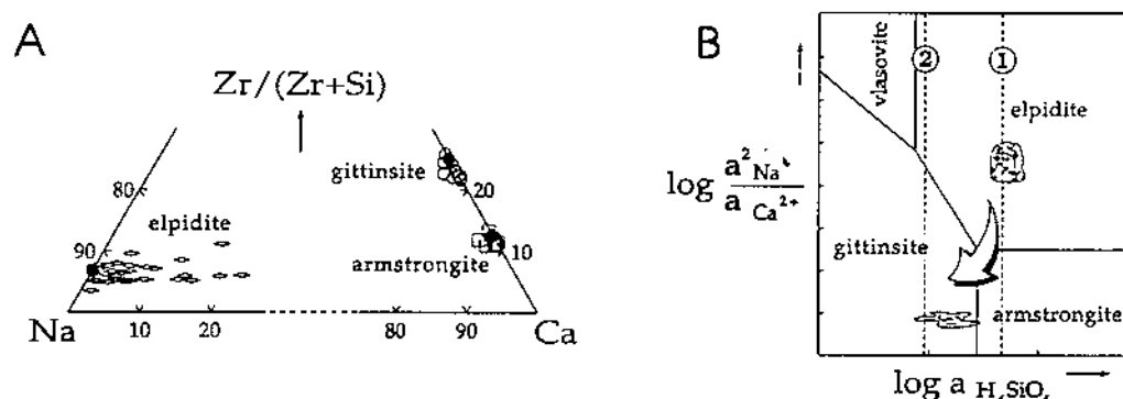
Fig. 2. A) A plot of the cation proportions in the Strange Lake zirconosilicate minerals calculated on the basis of 7 and 15 atoms of oxygen for anhydrous and hydrous species, respectively. Filled circles indicate end-member compositions. B) A schematic \log a_{Na^+}^2/a_{Ca^{2+}} vs. \log a_{H_4SiO_4} diagram showing zirconosilicate stability fields, and hypothetical compositions of unaltered elpidite-bearing granite and hydrothermal fluid. Lines 1 & 2 represent respective quartz saturation at deep and shallow levels in the drill hole.
