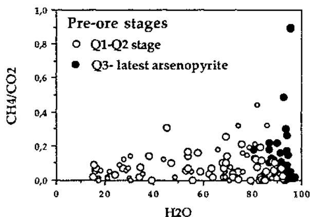
Fig. 1 : \text{CH}_4/\text{CO}_2 vs \text{H}_2\text{O} diagram applied to individual fluid inclusion compositions issued from microthermometric and Raman analyses (Corcoesto, Pino, Penedono, Tomino deposits).
