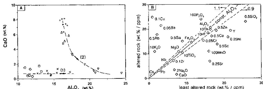
Fig. 2. (A) \text{Al}_2\text{O}_3 -CaO plots of cordierite-anthophyllite and associated rocks from the Tunaberg area; the diagram clearly shows two alteration trends: (1) from acid metavolcanics ( \circ ) and quartz-biotite schists ( \square ) to quartz-cordierite-anthophyllite-biotite schists ( \times ), and 2) from plagioclase-hornblende( \pm cummingtonite) rocks ( + ) to plagioclase-anthophyllite rocks ( \Delta ), and to cordierite-anthophyllite/gedrite rocks ( \nabla ). (B) Isocon diagram (Grant, 1986) showing outer zone hornblende-plagioclase( \pm cummingtonite) amphibolites versus inner zone cordierite-anthophyllite rocks. Oxides are plotted in weight percent, elements in ppm. Isocon line assumes constant alumina; elements with \sim 10 percent gain plot on 1.1 line, elements with \sim 10 percent losses plot on 0.9 line.
