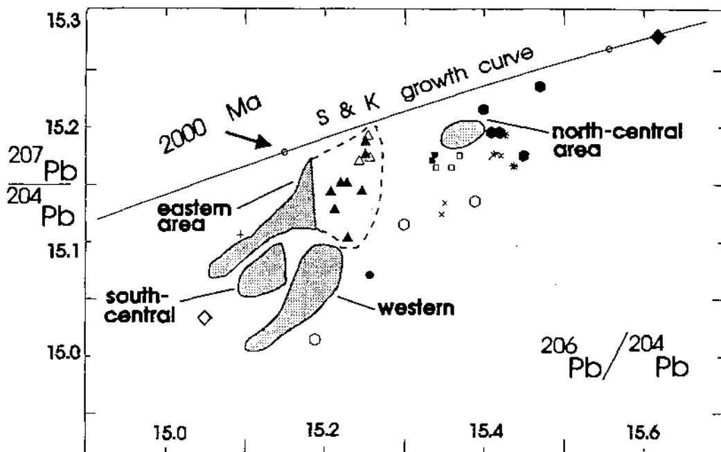
Fig. 1. Pb isotope data for epigenetic and VMS settings. + = Björkdal (Au), * = Tallberg (Au), x = Vindelgränsele (Au), filled circle = Vindelgränsele (VMS), open squares = Holmtjärn (Qz veins), filled squares = Holmtjärn (VMS), open polygons = Näsleden (veins), filled polygons = Näsleden (VMS), open triangles = Boliden (Au), filled triangles = Boliden (VMS), open rhomboeder = Barsele-arsenopyrite, filled rhomboeder = Barsele-jamesonite (Pb-sulfosalt).
