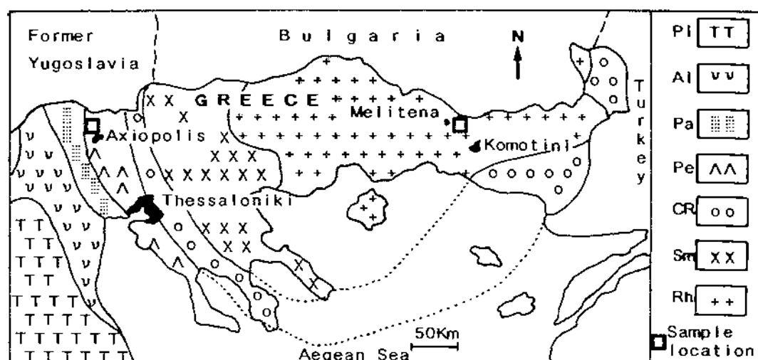
Fig. 1. Geotectonic sketch-map of a part of Northern Greece showing the sampling locations. Pl: Pelagonian zone, Al: Almopia zone, Pa: Paikon zone, Pe: Peonia zone, CR: Circum-Rhodope belt, Sm: Serbomacedonian massif, Rh: Rhodope massif.
