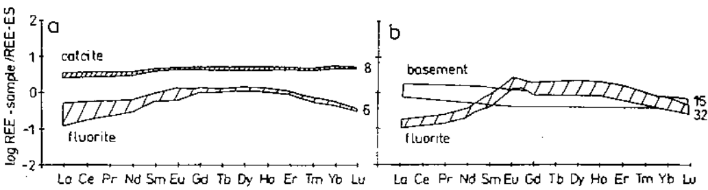
Fig. 1: REE distribution patterns of calcites and early fluorite (a) Gottesehre (# 9 in Fig. 1) and fluorites of the main fluorite stage (b) Wieden district (# 8 in Fig. 1). The light hatched band in Fig. 1b represents REE distribution patterns of gneisses and less-fractionated granites of the southern Black Forest. (Localities refer to Fig. 1 Franzke & Lüders, this issue).
