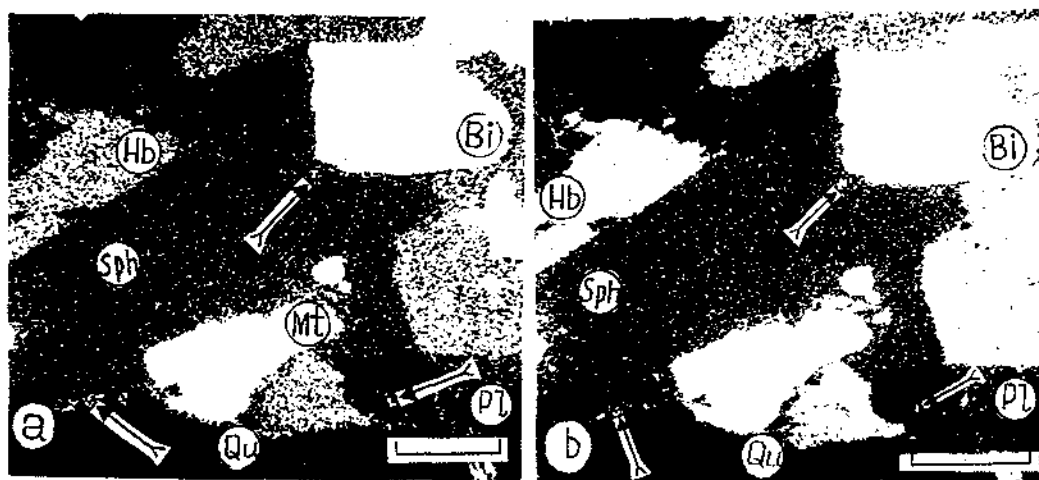
Fig. 1. X-ray images of the granite thin section. Mineral grains are marked: Mt — magnetite, Bi — biotite, Hb — hornblende, Sph — sphen, Ou — quartz, Pl — plagioclase. Au-Fe impurity inhomogeneities are pointed. a — FeK \alpha , exposure — 20 min, b — AuK \alpha , exposure — 72 min; scale bar = 20 \mu m.
