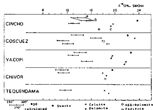
Figure 4. \delta^{18}\text{O} data of the carbonates and quartz from the studied deposits. The \delta^{18}\text{O} data in equilibrium with quartz and calcite are calculated at 250, 270 and 300°C. a: Fractionation factors of Bottinga and Javoy (1973), b: fractionation factor of Clayton and Mayeda (1972) applied to all the others quartz. 1= calcite stage I; 2= calcite stage II
