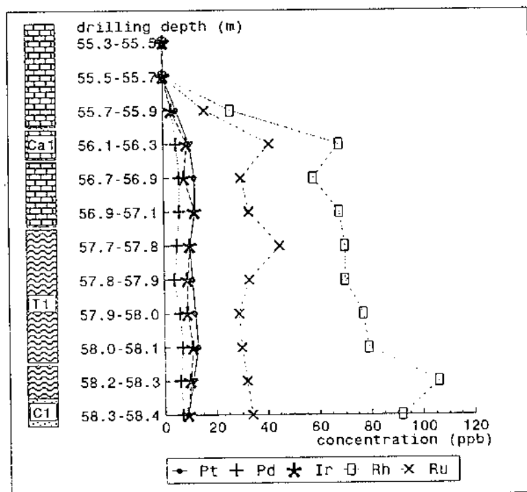
Fig. 3. Concentrations (ppb) and distribution of PGE in drill core 5 (Zechsteinkonglomerat (C1), Kupferschiefer (T1), Zechsteinkalk (Cal) ), N = 12.
