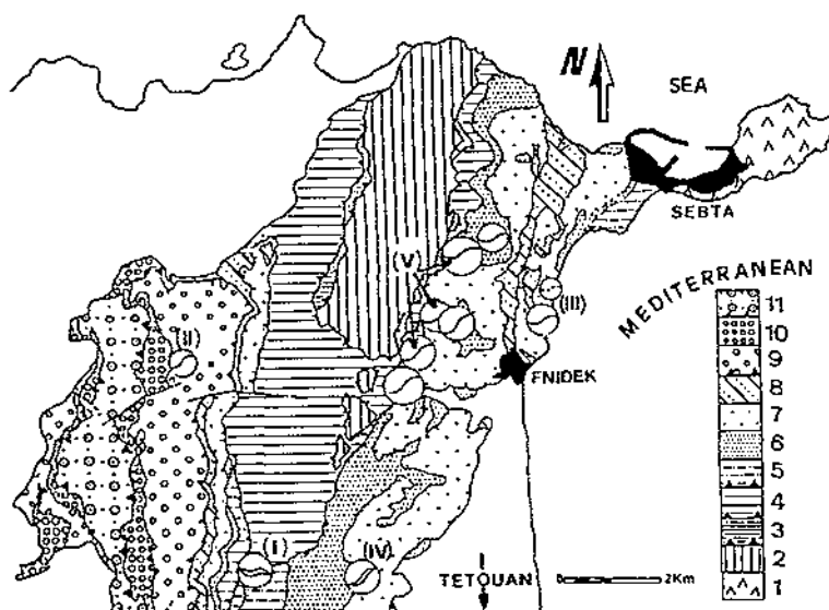
Fig.1: Geology and location of ore deposits in the Sebtides and Ghomarides tectonostratigraphic units, North Tetouan, Morocco. Sebtides: (1) Monte Hacho gneiss and serpentinite; (2) Beni-Mzala unit—schist (Permian), quartzite (Scythian), marble and dolomite (Anisian?); (3) Bouquette d'Anjera unit—schist (Permian), sandstone (Scythian), massive dolomite (Anisian); (4) Tizgarine unit—greywacke schist (Permian), quartzite (Scythian), massive calcareous dolomite (Anisian). Ghomarides: Akaili unit— (5) greywacke schist (Silurian), (6) highly deformed limestone (Devonian), (7) flysch (Carboniferous), (8) sandstone and conglomerate (Permo-Triassic); Koudiat-Tizian unit— (9) pelitic greywacke flysch (Devono-Carboniferous), (10) sandstone and conglomerate (Permo-Triassic); (11) Beni-Hozmar unit— "flysch" (Devono-Carboniferous), sandstone and conglomerate (Permo-Triassic). Ore deposits: I) Hriyech; II) Ain-Jir; III) Ain-Gharoq and Kurb-El-Hudoud; IV) Haïdra; V) Beni-Mzala district.
