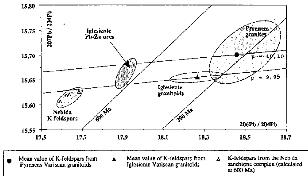
Figure 2 - Lead isotope plot for Iglesiasiente and Eastern Pyrenees formations
