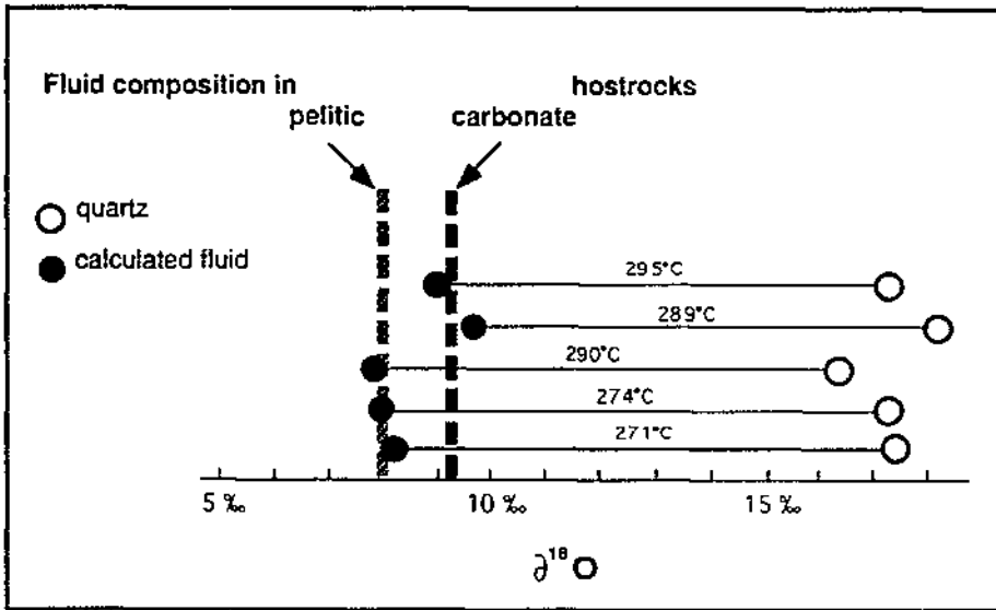
Fig.2. Isotope equilibrium temperatures of coexisting scheelite and quartz and calculated \delta^{18}\text{O} fluid composition in different host rock lithologies.
