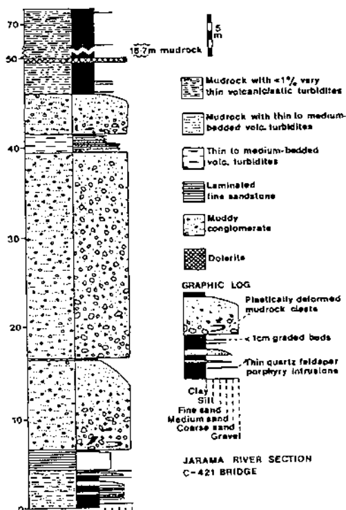
Figure 2 A measured section through an example of the resedimented hydro-clastic breccias to show the bed characteristics of these disorganised gravels.
