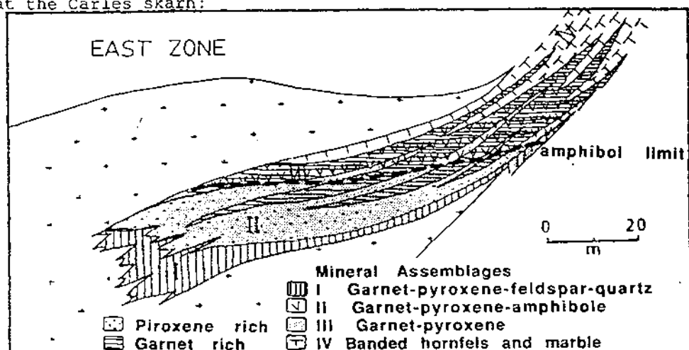
Fig. 2- Mineral assemblages among the two tongues of granodiorite in E part of the Carls deposit.
