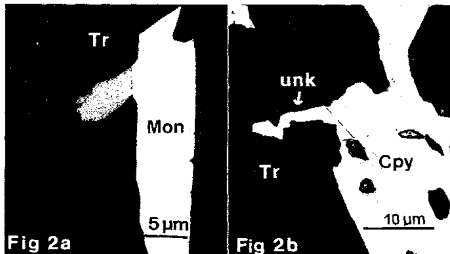
Figure 2 a. Photomicrograph of a large, moncheite grain (Mon) combined with pyrrhotite (Po) in a tremolite (Tr) matrix. b. Grain of unknown Pt-mineral (unk) combined with chalcopryrite (Cpy) in tremolite (Tr) matrix.
