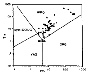
Figure 5. Yb-Ta tectonic discrimination diagram of Pearce et al. (1984) for the Porriño Peralkaline Complex
