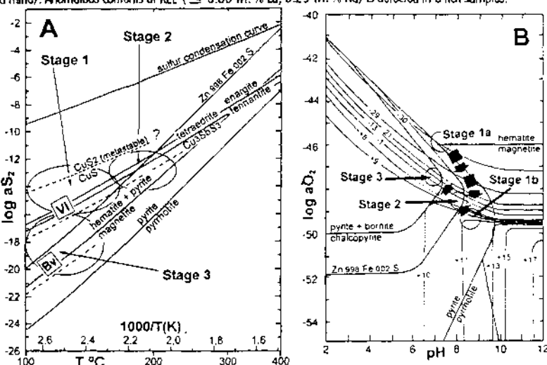
Figure 4.- A/ log P-T diagram showing sulfidation reactions for this study. Dashed lines represent equilibria for natural disulfides from these localities. Vi=villamaninite Cu_2Ni_3Co_1Fe_1S_7 , Bv=bravoite Cu_2Ni_3Co_1Fe_1S_7 . B/ log P-pH diagram at T=150 °C, I=3 and ES=0.01 showing the Fe-S boundaries and \delta^{34}S contours for H 2 S equiv. (Ohmoto 1972). \delta^{34}S values from this work (H 2 S at \delta^{34}S_{H_2S} = +9 ‰).
