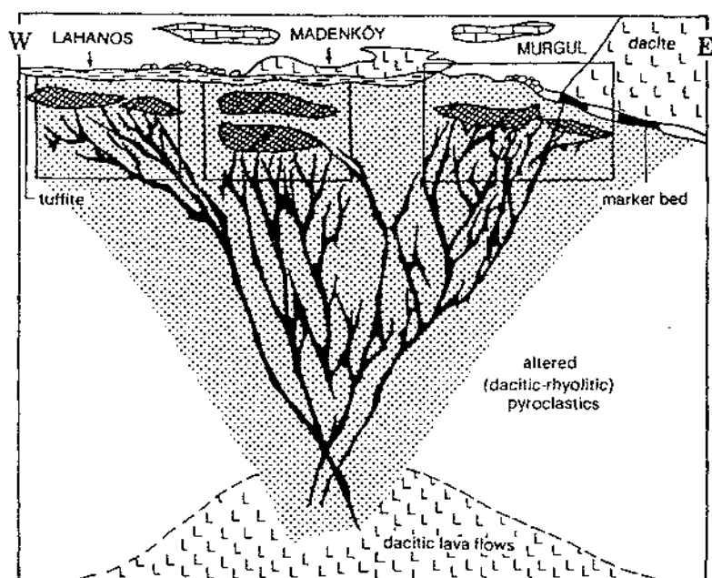
Fig. 2: Schematic presentation of the investigated ore deposits of the Murgul, Madenköy, and Lahanos in the East Pontic metallogenic province
