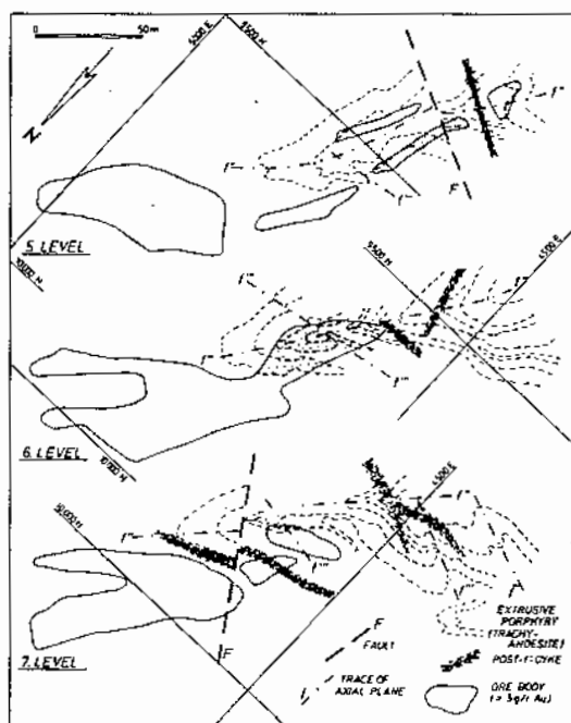
Fig. 3 Relationship between BIF (white), trachyandesite (stippled), dykes (dark shading), folds, faults and ore bodies (grey shading).
