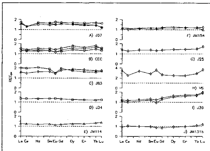
Figure 1.- Protolith normalized (GN) patterns of episyenites. Keys: (O) piroxene-, (□) amphibole-, (Δ) biotite-, (◇) chlorite- and (*) microcline-episyenites.
