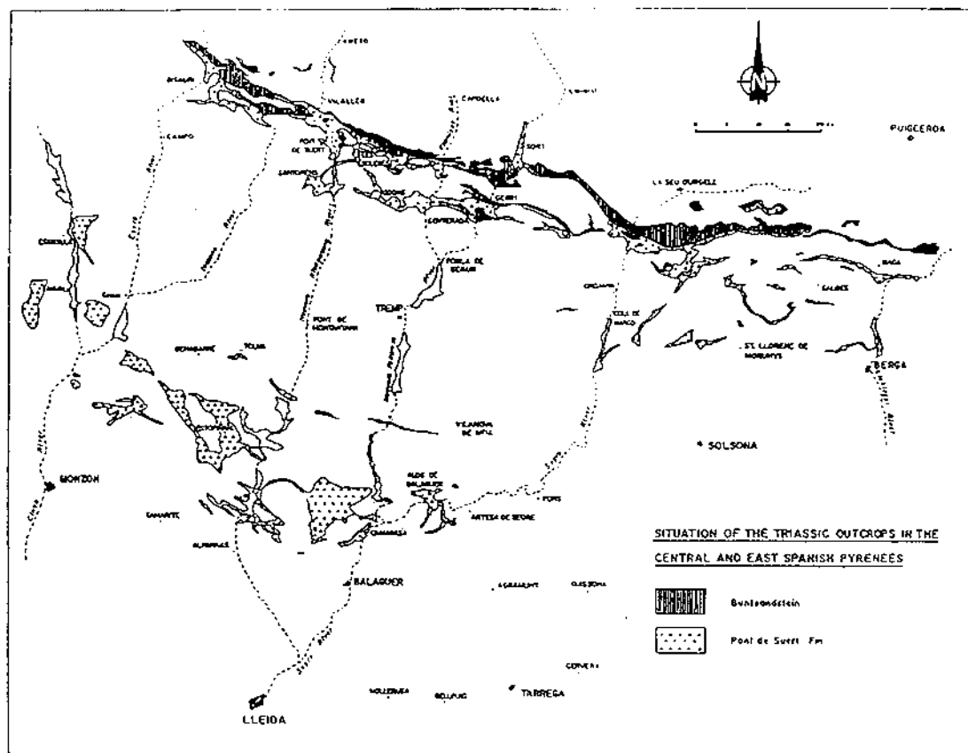
Figure 1. Situation of the triassic outcrops in the Catalan Pyrenees. The situated northward of the line Berga-Campo belong to the Upper thrust sheets of the MUÑOZ et al. (1986), those situated at the south, correspond to Lower thrust sheet.
