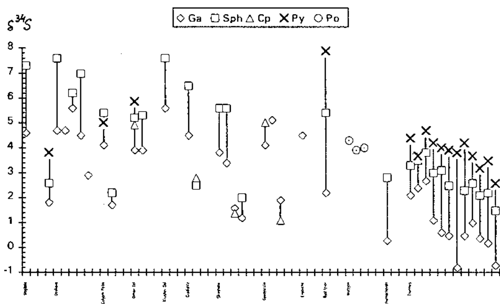
Fig.1 \delta^{34}S of sulphides from different deposits in the Madan district and the Thermes area
