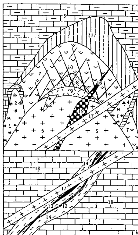
Fig. 2 Diagram showing the relationship between multiple phases of granitic rock and multiple periods of W-polymetallic mineralization
