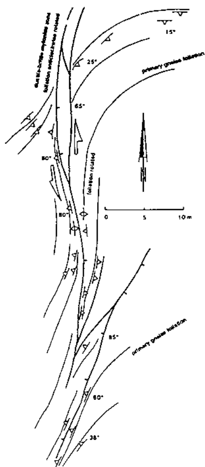
Fig. 2: Variscan structural pattern of the upper level of the "Caroline" mine NNE of Freiburg/Br. Sinistral transpressional shear zone.
