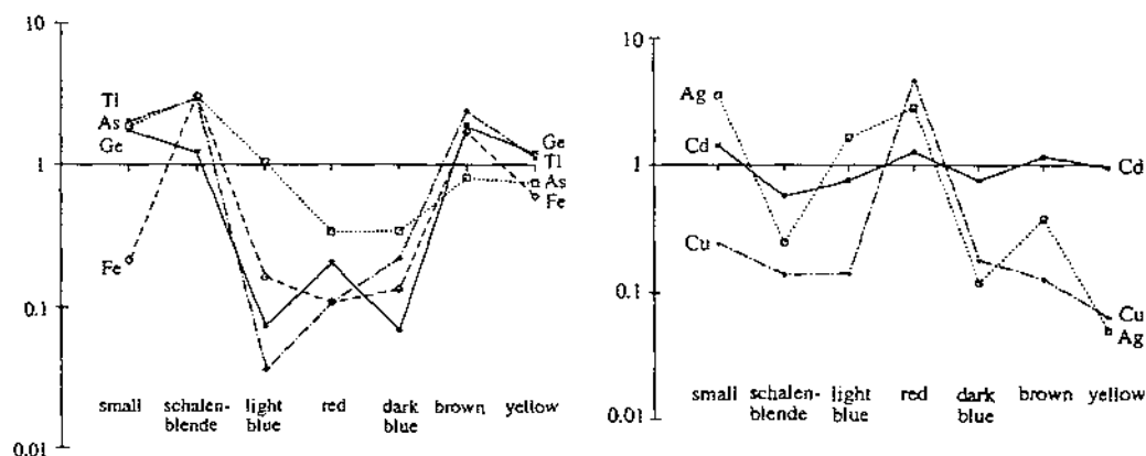
Fig. 4a/4b: Relative abundance of the trace elements (4a) Fe, As, Tl, and Ge as well as (4b) Cd, Cu and Ag in the succession of sphalerite types of the Drau Range.
