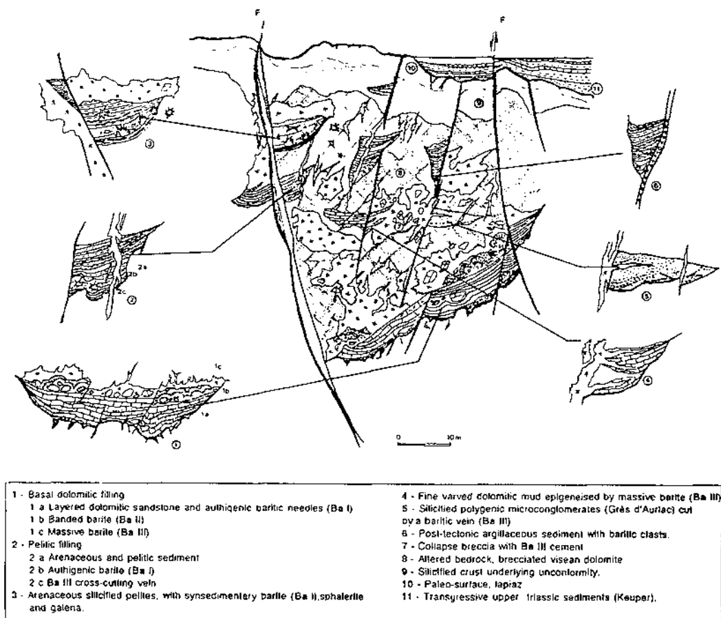
Fig. 1 . Karstic fillings spatial organisation in a baritic ore-body from the Mouthoumet Massif. (Giannoni, 1990, modified).
