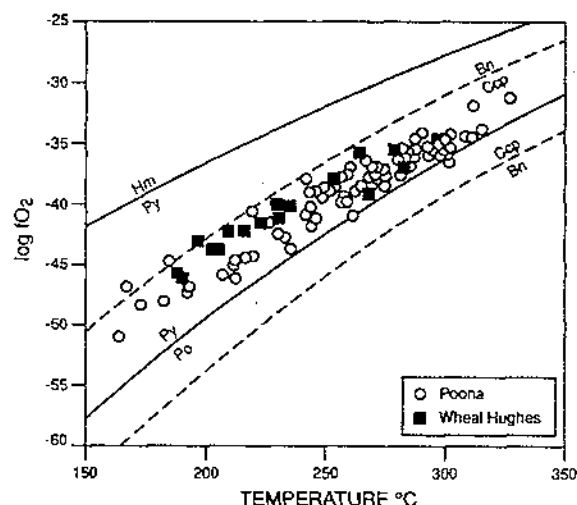
Fig. 4: Log fO_2 vs. T diagram showing chlorite data in relation to stability fields of pyrite (Py), pyrrhotite (Po), hematite (Hm), chalcopyrite (Ccp) and bornite (Bn). Calculated for pH=4.5.
