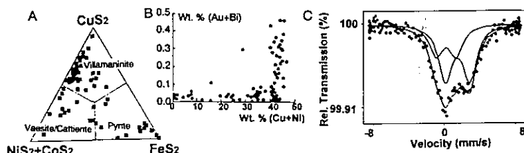
Figure 3.- Chemical characteristics of Providencia mine disulfides: A/ Plot of analysed points in the pseudoternary system \text{CuS}_2\text{-FeS}_2\text{-(NiS}_2\text{+CoS}_2\text{)} . B/ Correlation Au+Bi versus Cu+Ni. C/ Mössbauer spectra of ^{197}\text{Au} in villamaninite. A and B from Paniagua 1991, C from Friedl et al. 1991.
