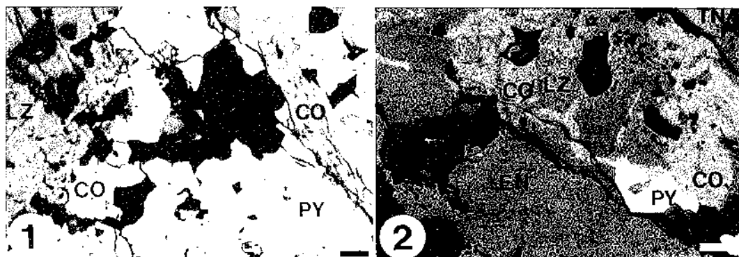
Figs.1+2 Colusite (CO) as inclusions in pyrite (PY) and as irregular network replacing luzonite/stibiolumonite (LZ). The zonal texture is well visible in Fig.2. EN,enargite; TN,tennantite. - Length of bar : 25 \mu m.
