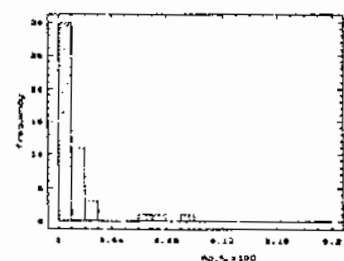
Fig.2 Histograms frequency and concentrations Ag (left) and Bi in native gold from rocks of Pervomaisky district. a) Au from the initially rock; b) Au from the weathering crust.
