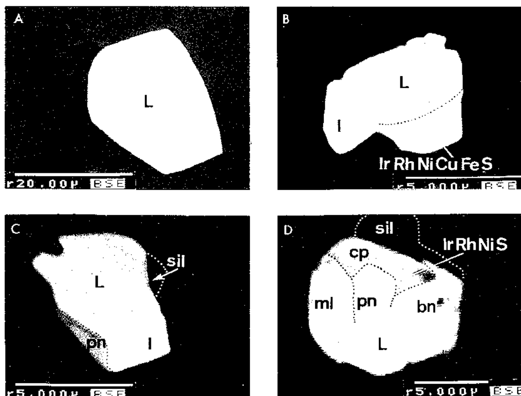
Figure 2.- Back-scattered images of single- and polyphasic inclusions in chromite. L = laurite, I = irarsite, cp = chalcopyrite, pn = pentlandite, bn = bornite, ml = millerite, sil = silicate.
