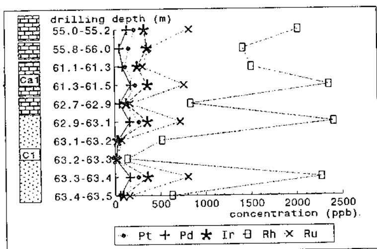
Fig. 2. Concentrations (ppb) and distribution of PGE in drill core 2 (Zechsteinkonglomerat (C1), Zechsteinkalk (Cal) ), N = 10.
