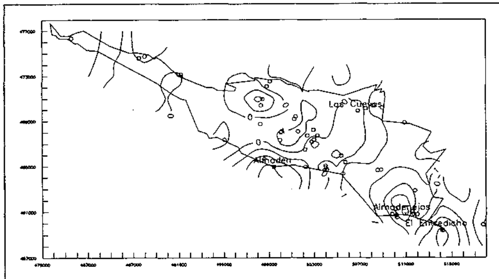
Figure 5.- Sketch map for the Rotated Factor 1 in the Almadén syncline. Irregular line: Criedero quartzite. Symbols for the samples, as in figures 1 and 2. Border: Lambert coordinates.
