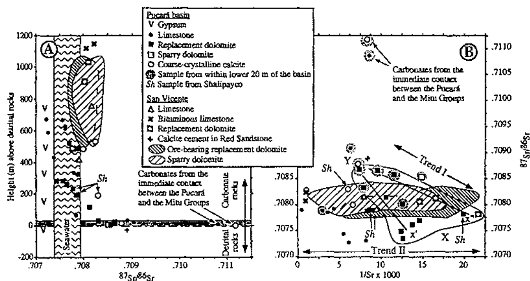
Figure 2 - Height vs. ^{87}\text{Sr}/^{86}\text{Sr} ratios and ^{87}\text{Sr}/^{86}\text{Sr} ratios vs. 1/\text{Sr} \times 1000 (ppm -1 ). San Vicente data is from Fontboté and Gorzawski (1990) and Upper Triassic to Lower Jurassic seawater Sr range is from Koepnick et al. (1990).
