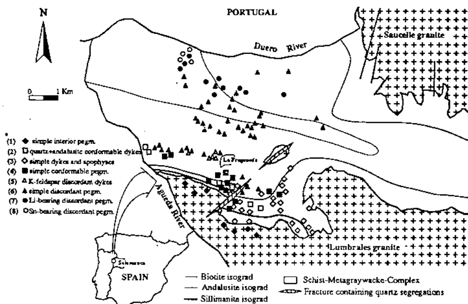
Fig. 1: Distribution of the pegmatite groups differentiated in the Fregeneda area. (*numbers as in "Geology of pegmatites").
