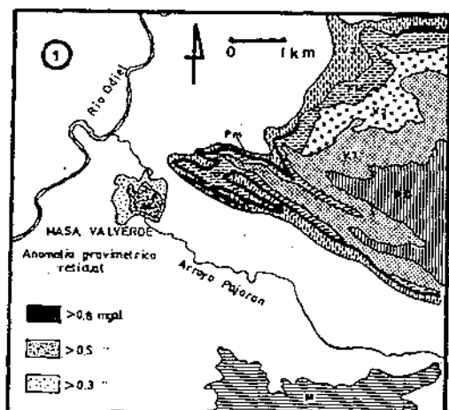
Fig 1.- Location of the gravity anomaly of Masa Valverde deposit (Huelva, Spain). Fig 2.- Cassiterite (dark grey, center) and pyrite (white) crystals in sphalerite (PPL, =N). Fig 3.- Two types of fine grain zircon crystals in chloritite (PPL, +N).
