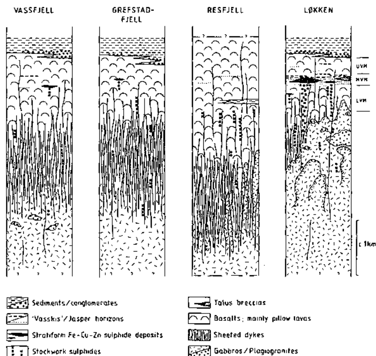
Fig. 1. Generalized sections of the Vassfjell, Grefstadfjell, Resfjell and Løkken ophiolite fragments. Question marks denote unexposed bases or tectonic boundaries.
