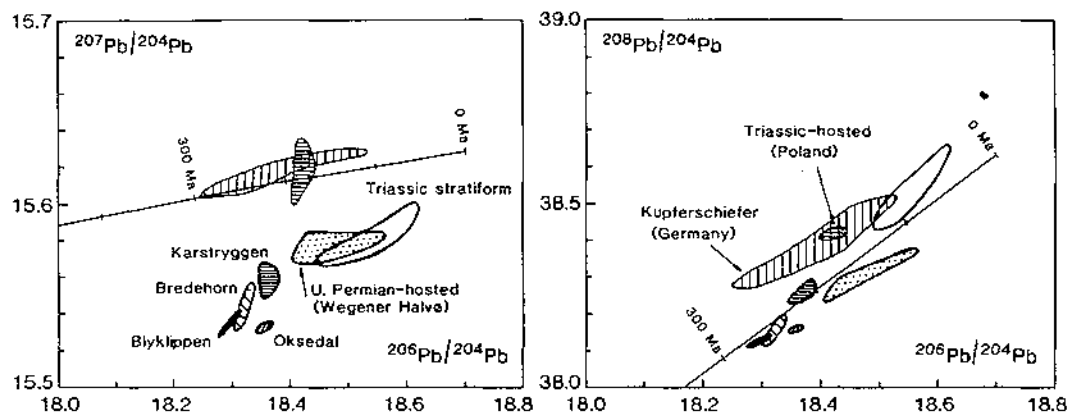
Fig. 2. Lead isotope compositional fields for sediment-hosted base metal occurrences in the Jameson Land basin compared to data for the Permian Kupferschiefer in Germany (Wedepohl et al., 1978) and Pb-Zn ores in the Triassic Muschelkalk in Poland (Zartman et al., 1979). Terrestrial lead isotope growth curves from Stacey & Kramers (1975).
