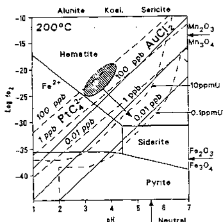
Fig.3: Log fO_2 -pH diagram, showing the distribution of iron phases, and the solubility of U oxides, AuCl_2 , and PtCl_4^{2-} in solution at 200°C. Heavy arrows on the right ordinate mark the position of the hematite+magnetite and Mn_3O_4 + Mn_2O_3 redox buffer assemblages. The hatching indicates the possible pH and oxidation state of the original ore fluid, and the light arrow a possible reaction path (from Mernagh, 1992).
